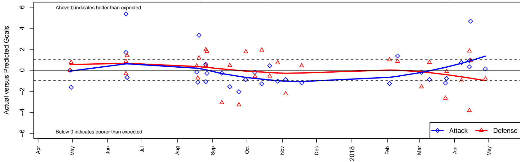
Cascade FC Green B05 Dots are actual minus expected GF (blue circles) and GA (red triangles). Blue line is smoothed change in attack strength. Red is smoothed change in defense strength.
